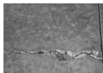
Fig. 1: Performing a concrete condition assessment can expose the presence of bugholes, honeycombs or cracking prior to coating application. Photos courtesy of SSPC.
