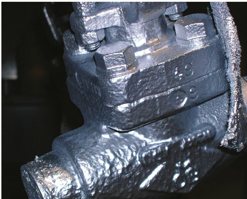
Fig. 2: Stippled, wavy appearance of the coating on a small valve indicates airless spray application and an attempt to control DFT by repeatedly triggering the airless gun.
