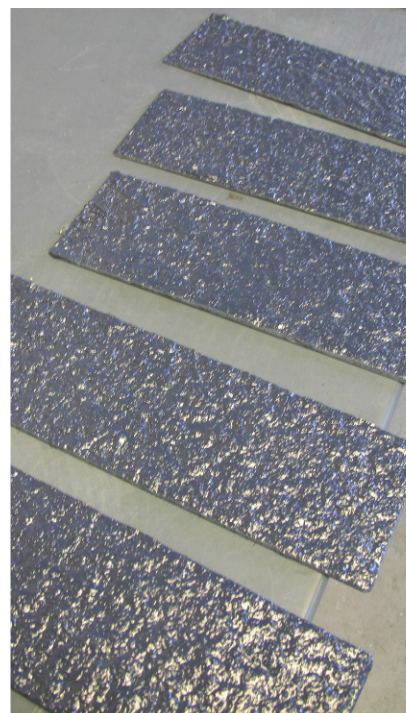
Fig. 6: Test strips from material testing show the consistent mil build achieved from spraying non-skid materials with a two-ball piston pump designed for mortars. Photo courtesy of C.H. Reed.
