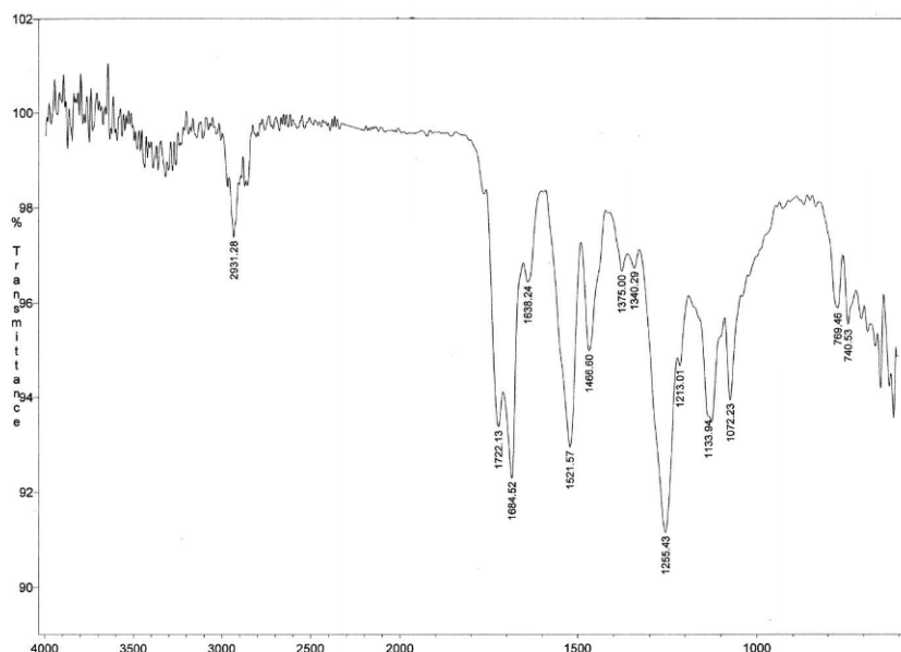
Fig. 2: The infrared spectrum of the dull top-coat from one of the core samples, showing it to be a polyurethane.
