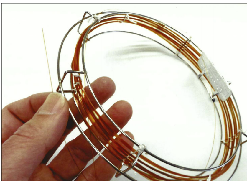
Fig. 1: A modern 30 meter capillary column. Note how thin and flexible the fused silica tubing is. All images courtesy of the author.
