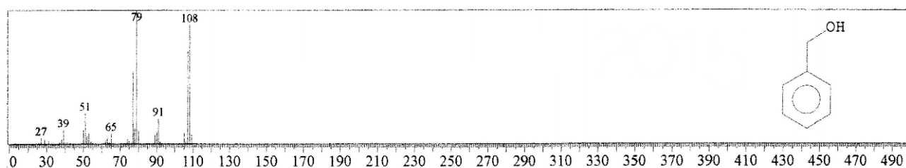
Fig. 6: The mass spectrum of benzyl alcohol, a common ingredient in many epoxy coatings.
