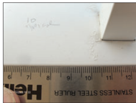
Fig 3: (Case 2) Typical appearance of filiform threads on powder coated aluminum at a picket penetration of the bottom rail. Not to scale.
