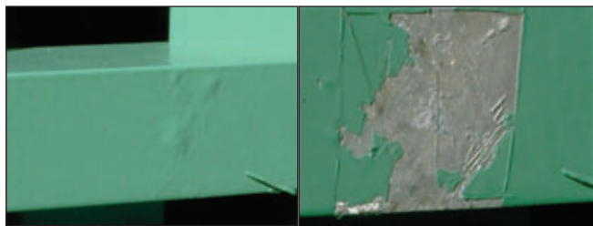
Fig 6: (Case 3) Intact coating blisters on a railing section prior to removal of the coating (left) and the appearance of the substrate (right) with confined spots of corrosion product.
